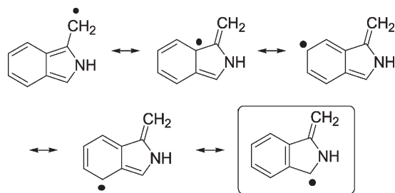
Figure 7. Resonance forms of the 1-methyl-2 H -isindole radical
